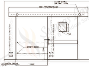
Single Door
