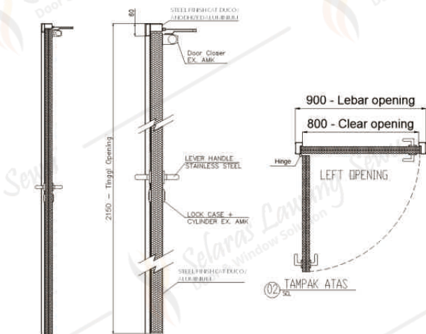
01 TAMPAK SAMPIING
